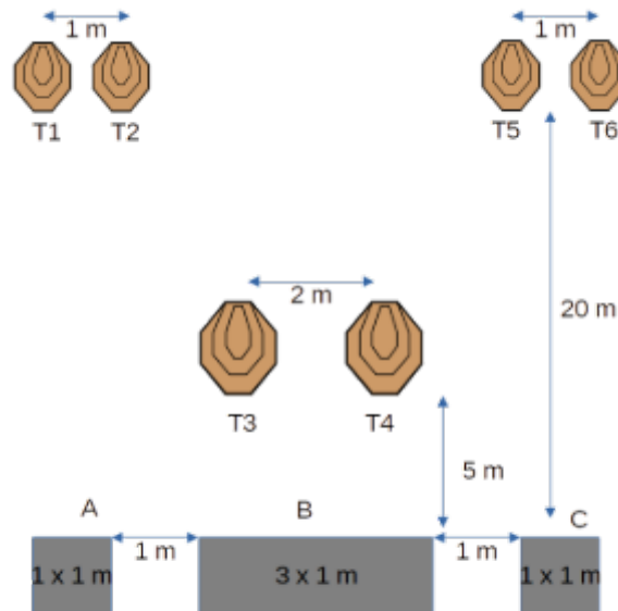
4 IPSC mini targets at 20 m (1 m from ground to bottom of target) 2 IPSC targets at 5 m (0.5 m from ground to bottom of target)
